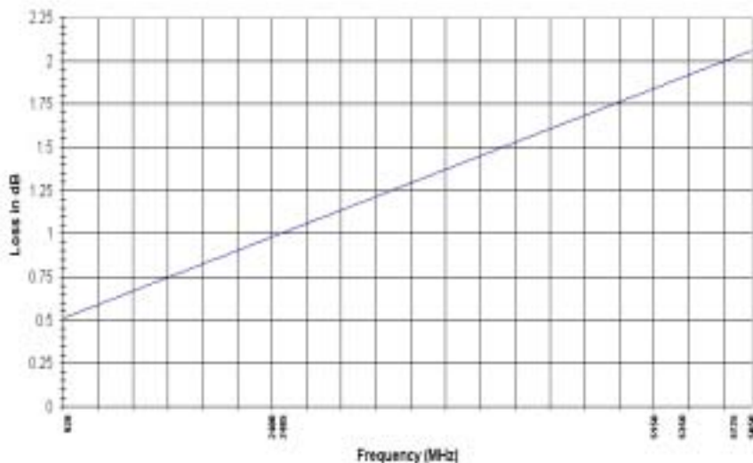
MW-RD Loss Versus Frequency
